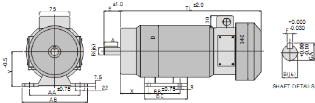
(M30-T, M3-T, M5-T, M7-T) Foot Mounting
