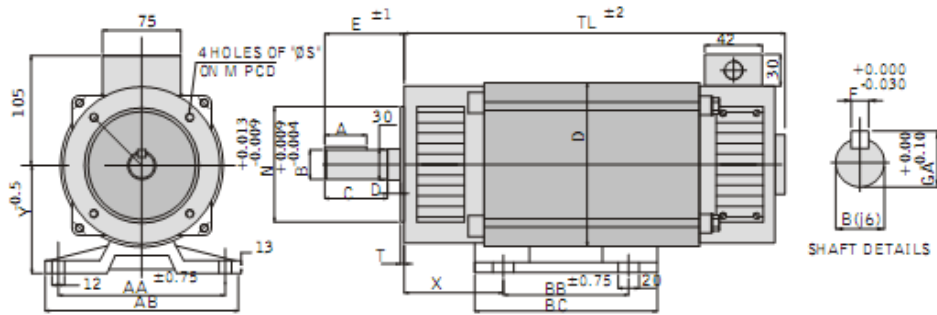
(S2N-F & S2N-T, V1-T, V2-T, V3-T)
