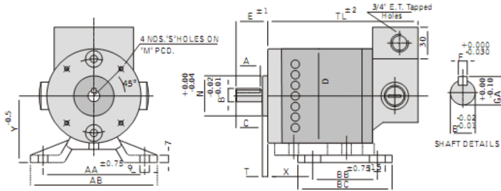
(M30-L, M3-L, M5-L & M7-L) Face Dimensions
