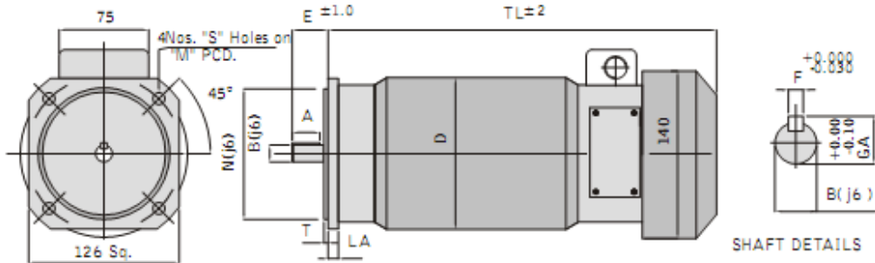
(M30-71B5, M3-71B5, M5-71B5, M7-80B5) IEC Flange
