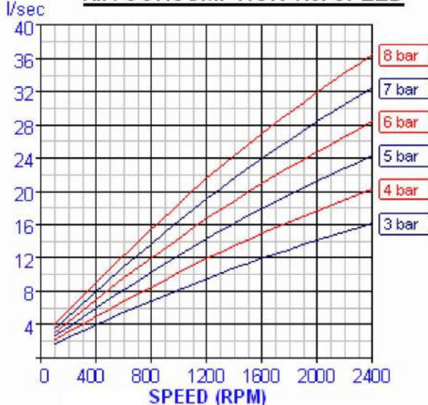
Free air AIR CONSUMPTION v.s. SPEED
