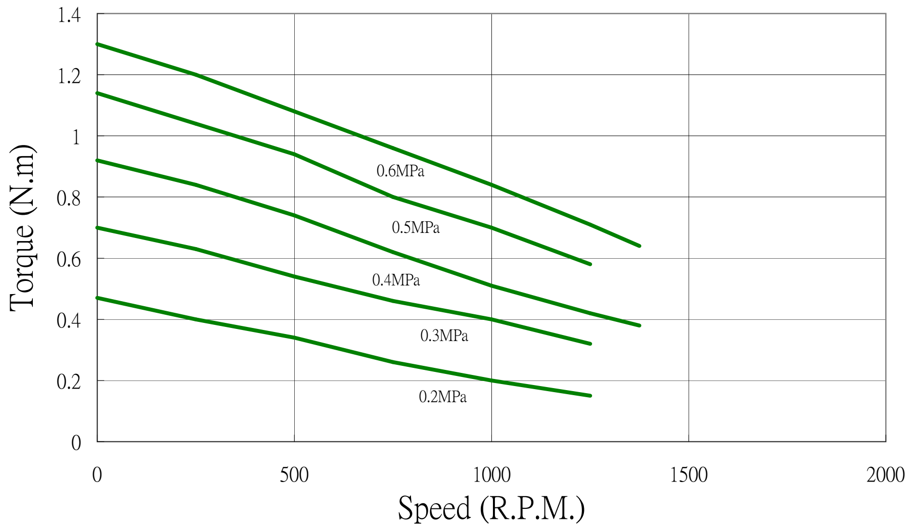
M1 Torque v.s. Speed
