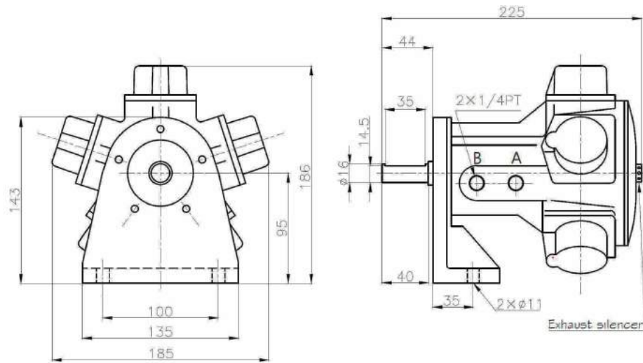
M5-L Foot
