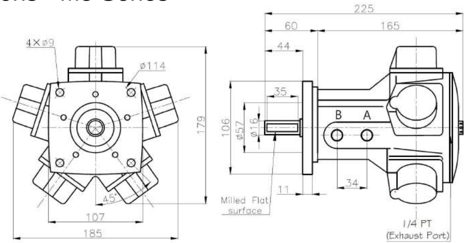
M5-F Face
