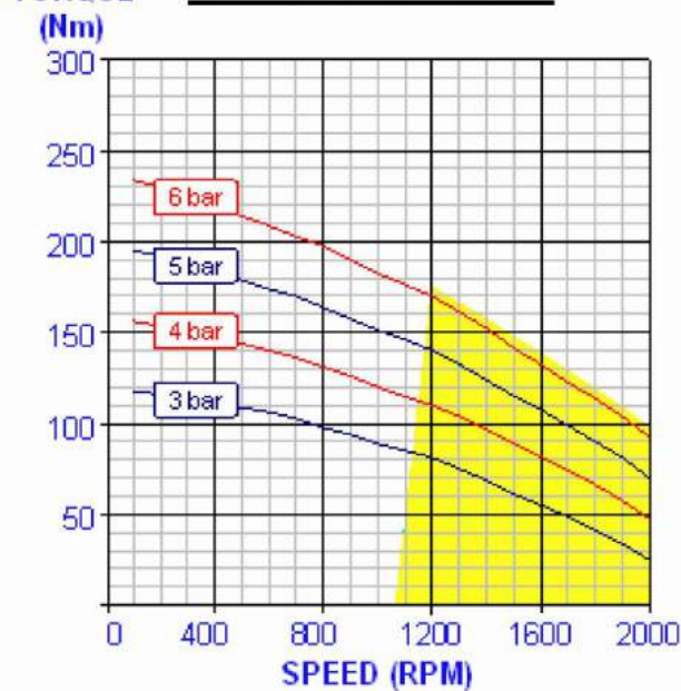
TORQUE v.s. SPEED
