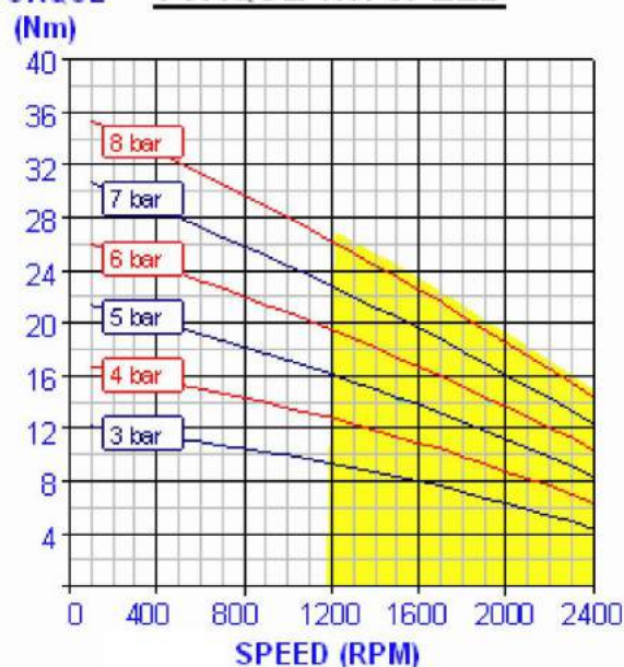
TORQUE TORQUE v.s. SPEED
