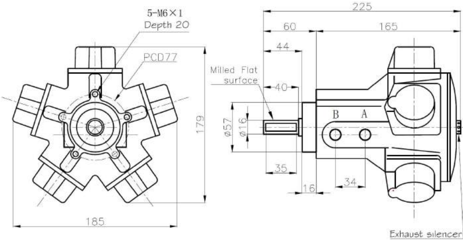
M5-T Standard
