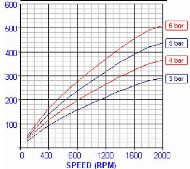
Free Air AIR CONSUMPTION v.s. SPEED
