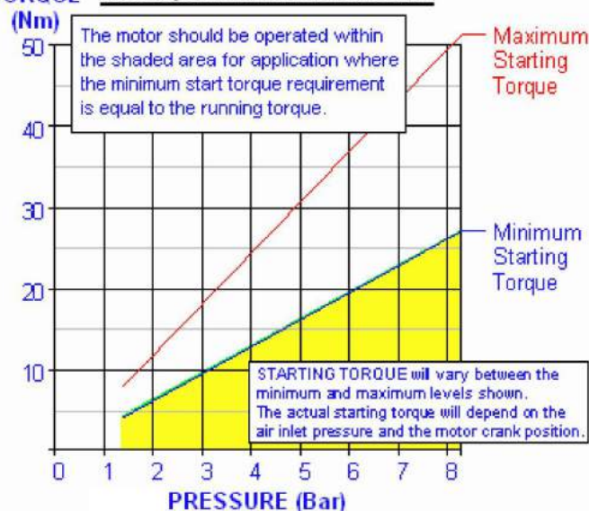
TORQUE TORQUE v.s. PRESSURE
