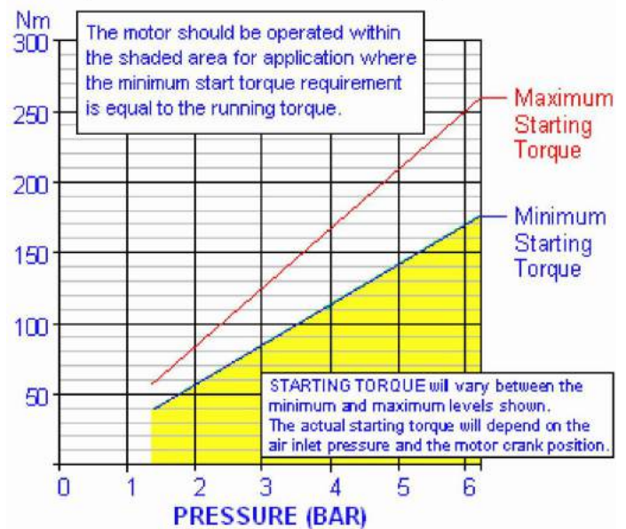
TORQUE v.s. PRESSURE
