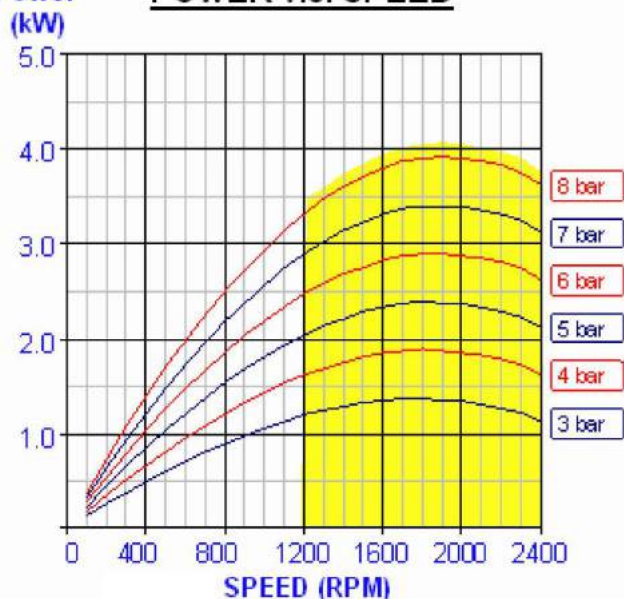
Power POWER v.s. SPEED
