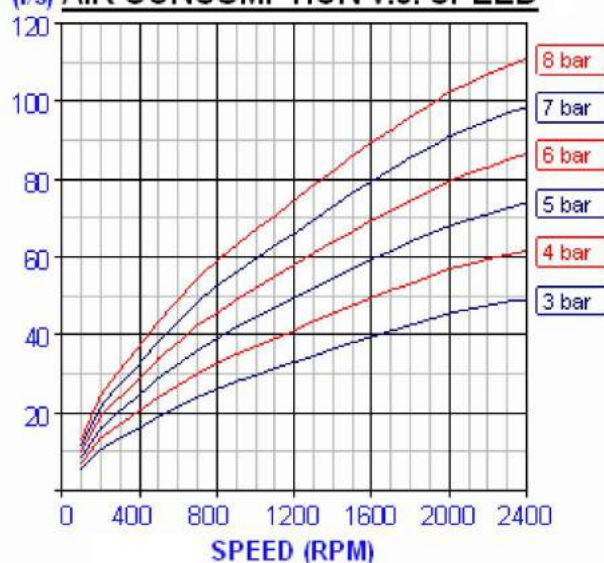
Free Air AIR CONSUMPTION v.s. SPEED
