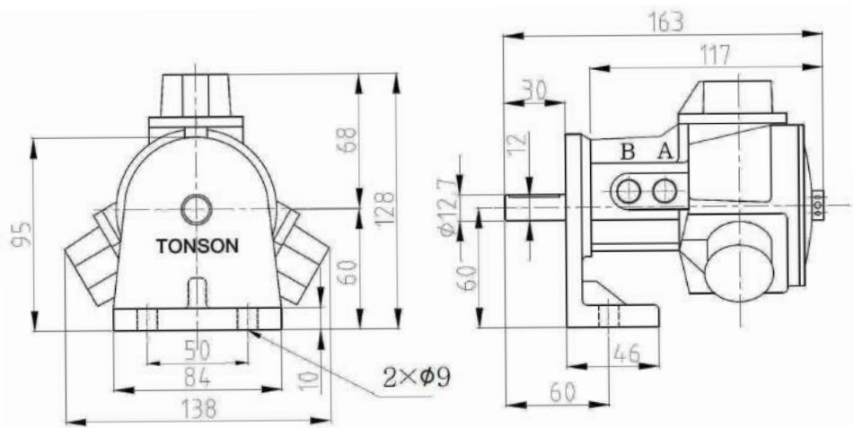
M2-L Foot
