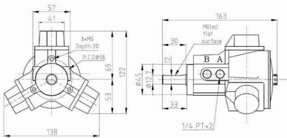
M2-T Standard
