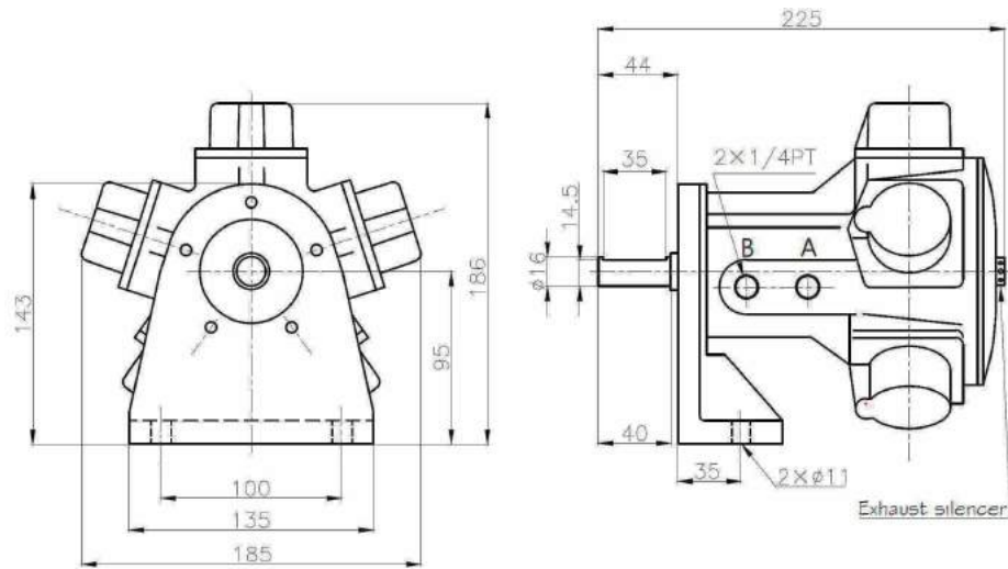
M5-L Foot
