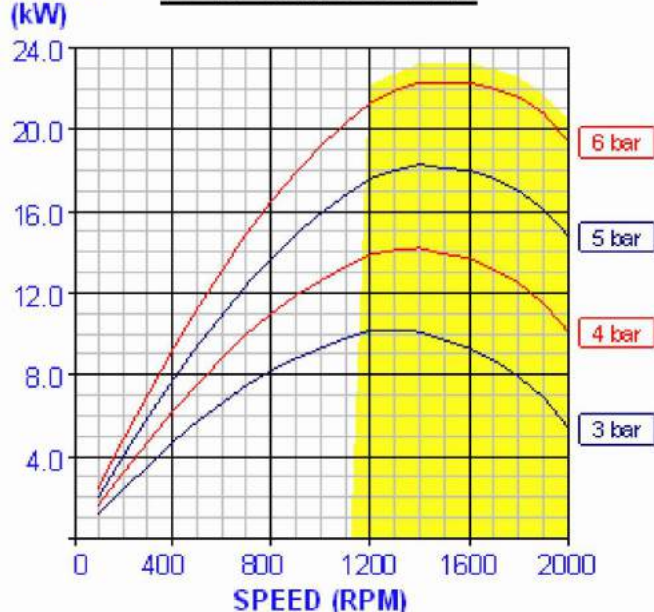
POWER v.s. SPEED
