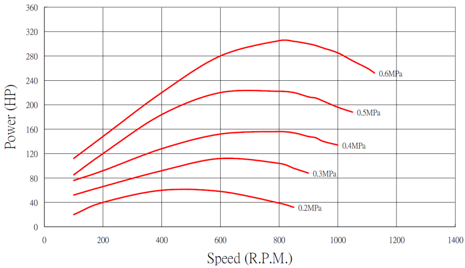
M5 Torque v.s. Speed
