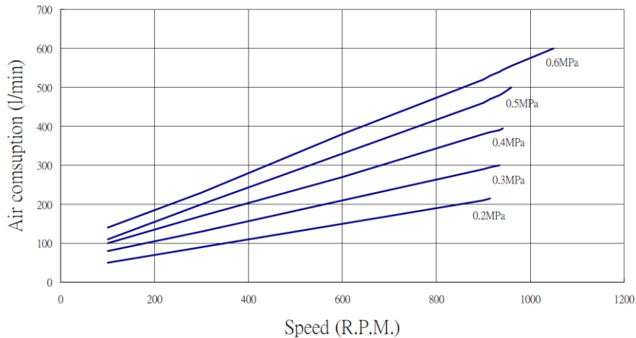
M5 Air consumption v.s. Speed
