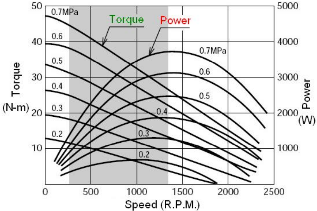
POWER & TORQUE v.s. SPEED
