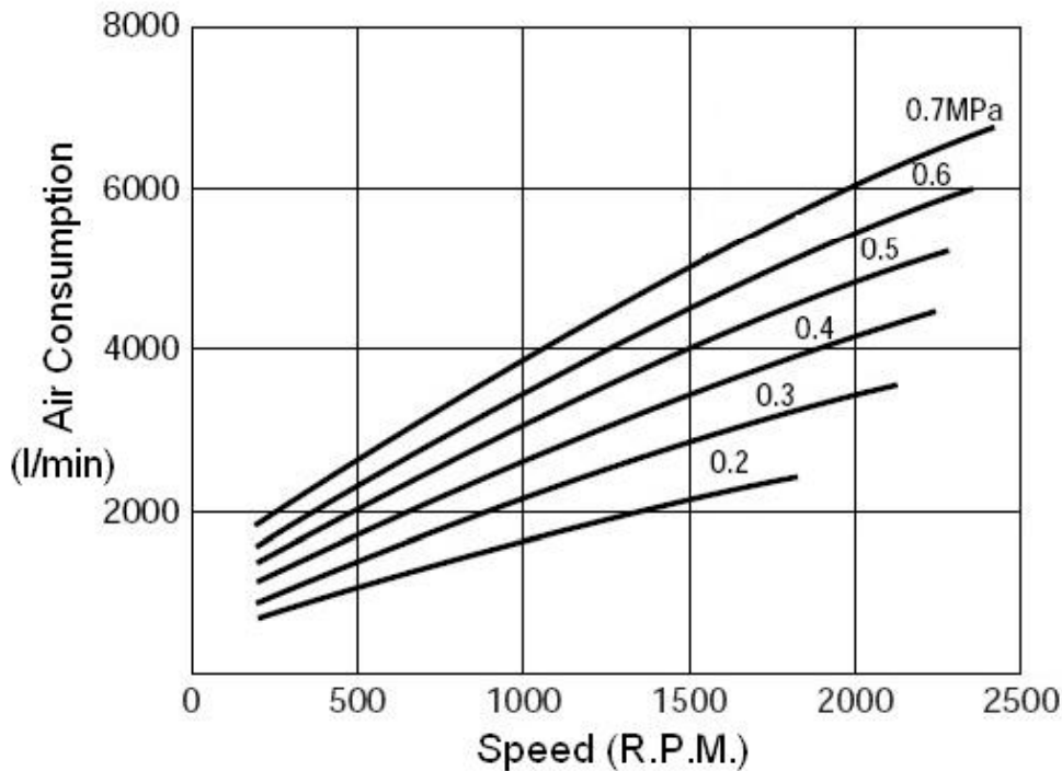
AIR CONSUMPTION v.s. SPEED
