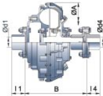
Technical Specification and Dimension Table for HF/ HFD/ HF-DX couplings
