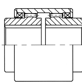
SLEEVE TYPE
