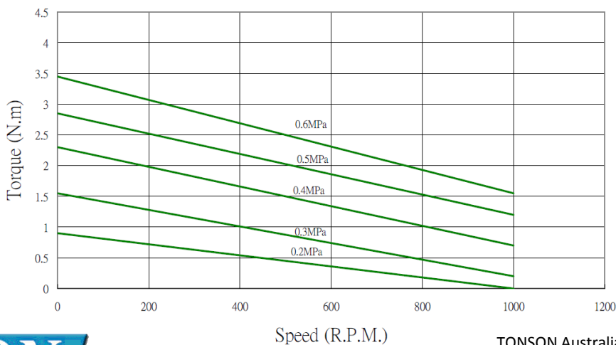
M3 Torque v.s. Speed
