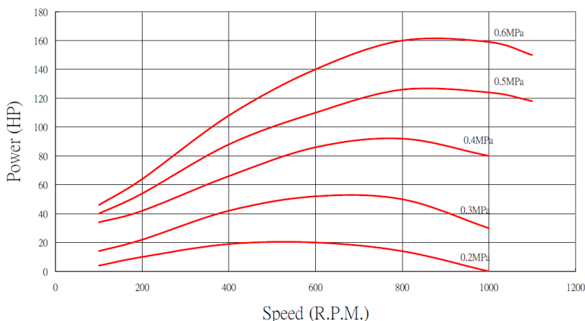
M3 Air consumption v.s. Speed
