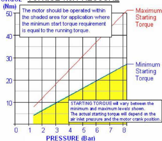
TORQUE v.s. PRESSURE
