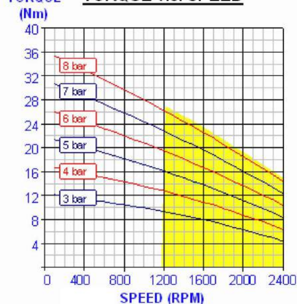
TORQUE v.s. SPEED
